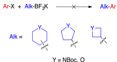
Scheme 3. Cross-Coupling of Nonaromatic Heterocyclic Trifluoroborate Salts with Aryl Halides
